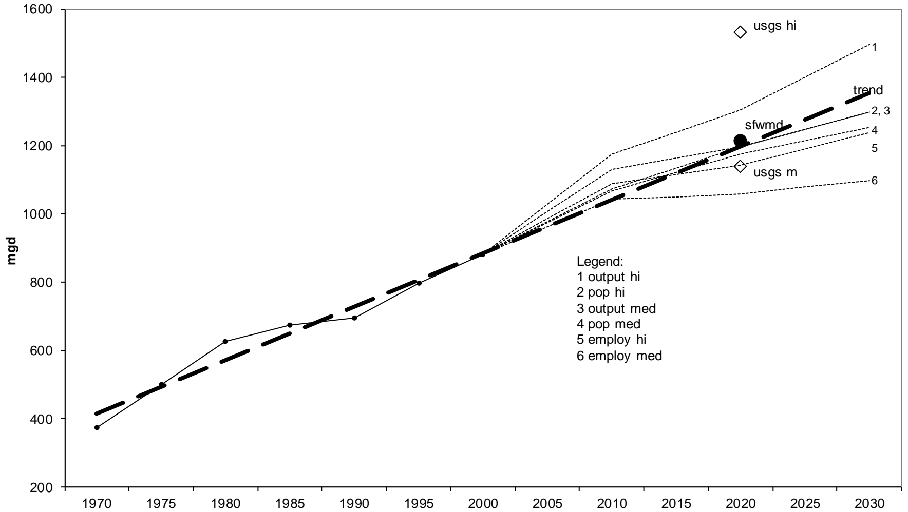
Figure 3.1 Projections of Public Water Supply: Lower East Coast
